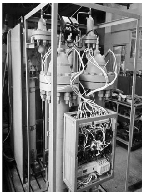
Fig. 7. Laboratory model of hydrogen energy accumulator
